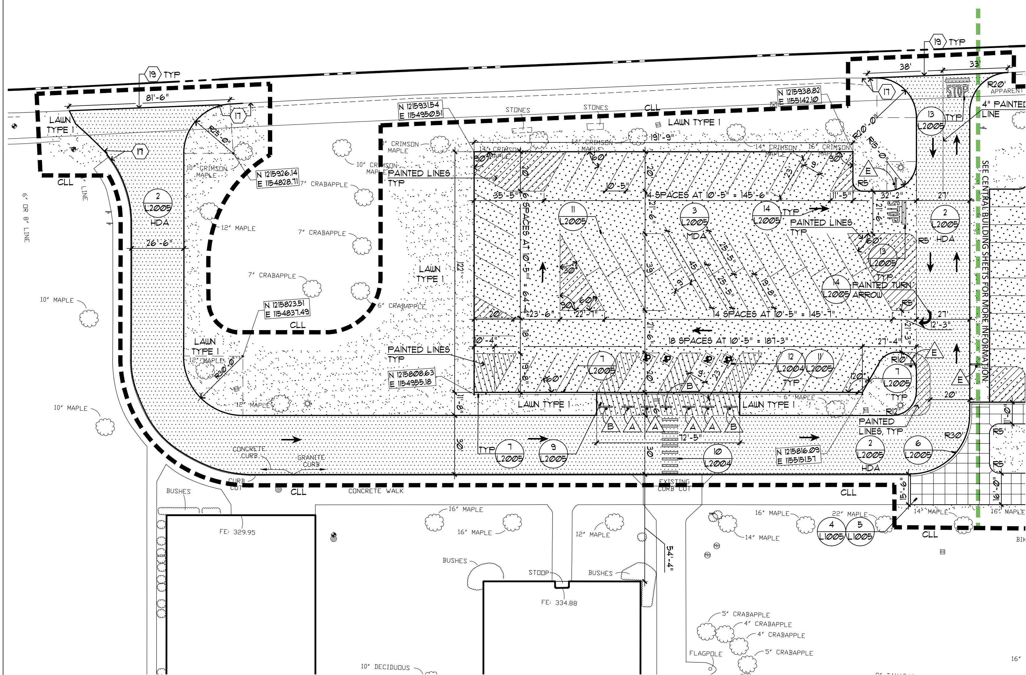
LAYOUT PLAN
