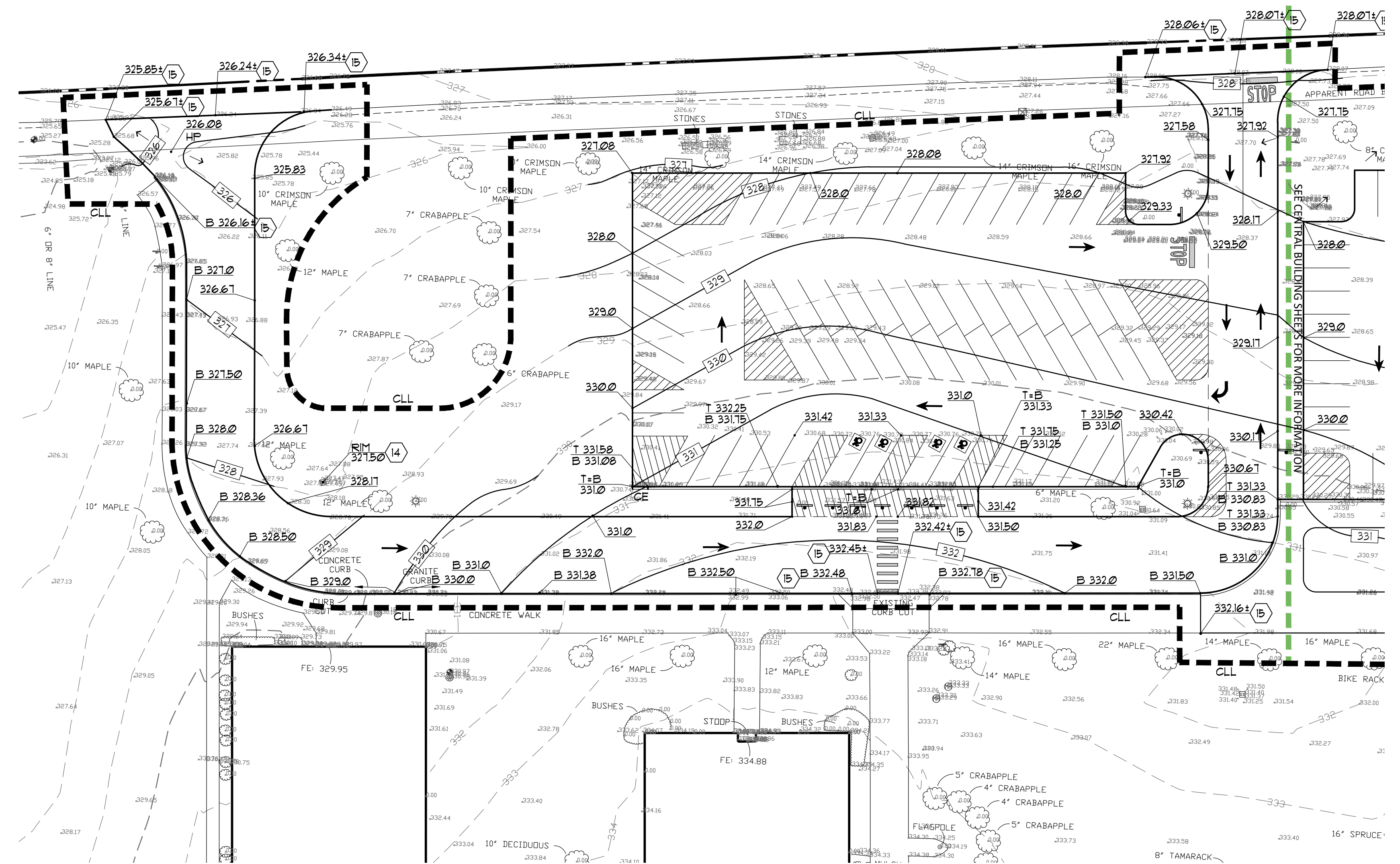
GRADING AND DRAINAGE PLAN
